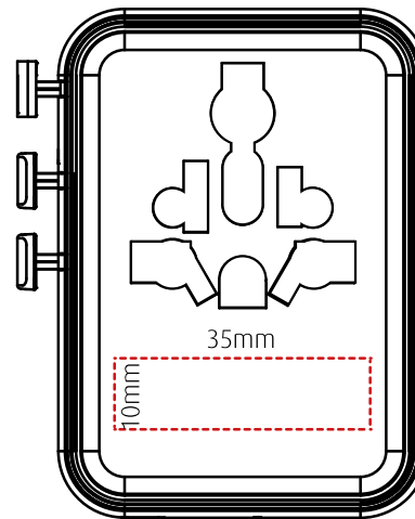
Below multi socket (UK pins)
